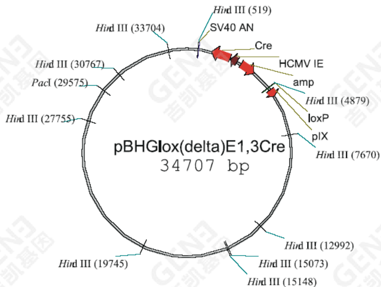
Fig. 3 pBHGllox ΔE1, 3 Cre 质粒图谱
